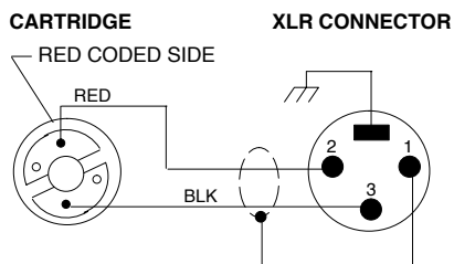
SM10A WIRING DIAGRAM
