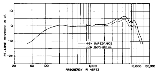
FREQUENCY RESPONSE
