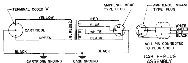
INTERNAL CONNECTIONS
