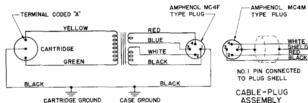
INTERNAL CONNECTIONS
